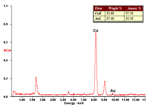
Fig.S1 EDX spectrum of the Au/Cu 2 O HGS of adding 1.5 mL HAuCl 4
