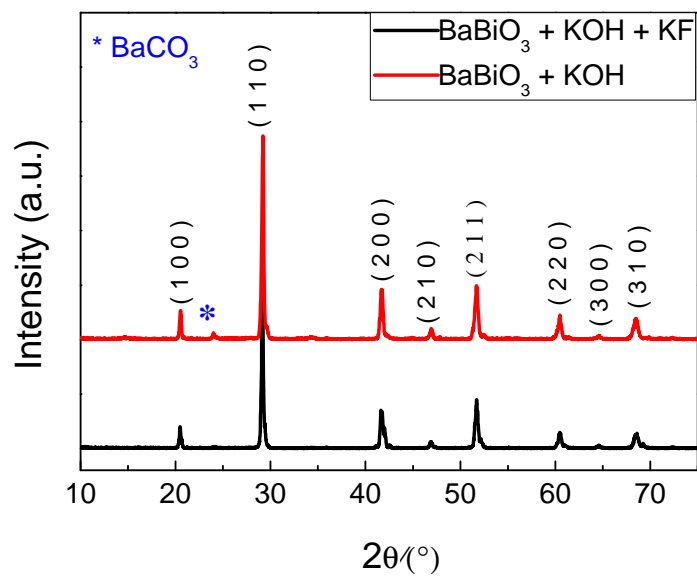
Fig.S1 Powder X-ray diffraction pattern of \text{Ba}_{1-x}\text{K}_x\text{BiO}_3 with different starting flux composition
