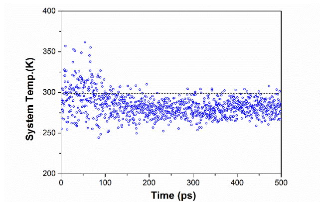
Fig. S1 Fluctuations of the system temperature with the time evolution of the 500 ps RMD simulation.
