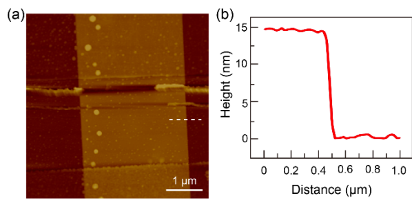
Fig. S1 The corresponding AFM images and height profiles of FET transistor of the Fig. 4d in the main text.
