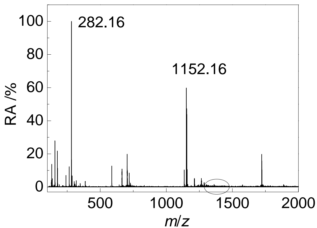
Fig.2 ESI mass spectra of the simple mixed solution of \beta -CD and 18C6 (molar ratio 1:1)
