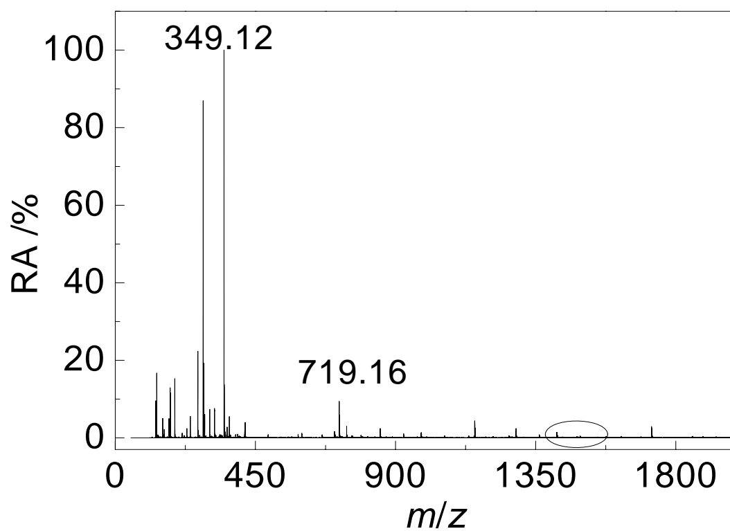
Fig.S2 ESI mass spectra of the simple mixed solution of \beta -CD and 18C6 (mass ratio 1:1)
