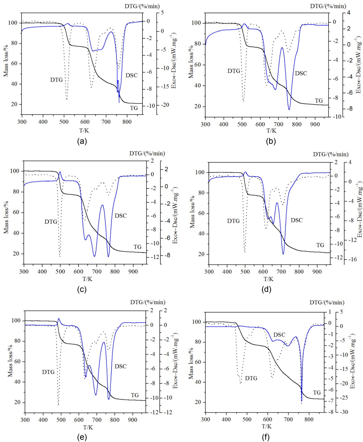
Fig. S1 The TG-DTG-DSC curves of the complexes 1–6 (a–f).
